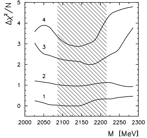
Fig. 17. The reduced \chi^2/N for the N(2170)D_{13} mass scan. 1: \chi^2/N for d\sigma/d\Omega ( \Lambda K^+ ) (CLAS, SAPHIR, 300 data points); 2: \chi^2/N+1 for \Sigma K (CLAS and SAPHIR, 390 data points); 3: \chi^2/N+2 for \Lambda K^+ recoil polarisation (CLAS, 46 data points), and 4: \chi^2/N+3 for \gamma p \rightarrow \pi^+ n (86 data points).
