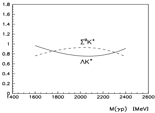
Fig. 2. Energy-dependent normalisation factor. The solid line is for the \Lambda K^+ data and the dashed line is for the \Sigma K data. The fit result was multiplied by the factor before it was compared with the SAPHIR data.
