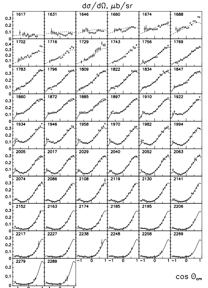
Fig. 4. The angular distributions as a function of W for \gamma p \rightarrow \Lambda K^+ , CLAS data. The prediction for the region where data were not used in the fit is shown as dashed lines.
