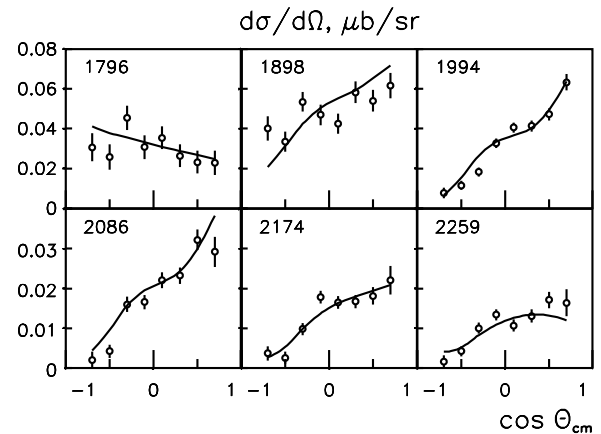
Fig. 13. Angular distributions for K^0\Sigma^+ , CLAS data.
