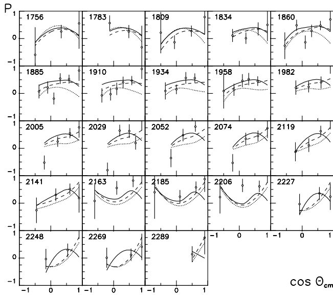
Fig. 11. Recoil polarisations for K^+\Sigma^0 , CLAS data. The solid curves are results of the fit. The dashed curves correspond to the solution without N(2170)D_{13} and the dotted curves to the solution without (1840)P_{11} .
