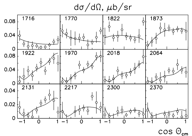
Fig. 14. Angular distributions for K^0\Sigma^+ , SAPHIR data.
