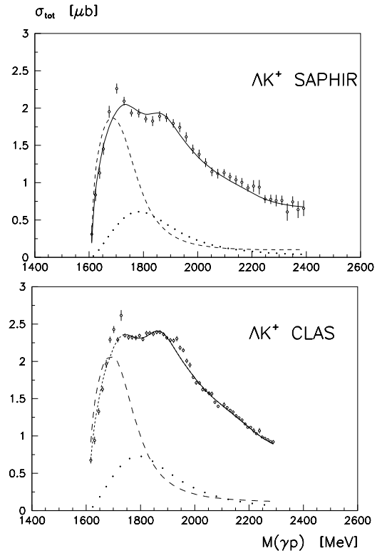
Fig. 1. The total cross-sections as a function of W = M_{\gamma p} for for \Lambda K^+ photoproduction measured by SAPHIR [12] and CLAS [13]. The solid curves are results of our fit. The dashed lines show the contribution from S_{11} K -matrix amplitude; the dotted lines show the contribution from P_{13}(1720) . The prediction of the total cross-section in the region where data were not used for the fit is shown as short-dashed line. The discrepancy at M_{\gamma p} \sim 1.7 GeV is discussed in sect. 2.1.
