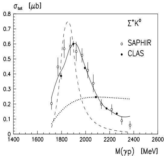
Fig. 12. Total cross-sections for K^0\Sigma^+ photoproduction. The solid curve represents our fit. The SAPHIR cross-section is shown as open circles. For the CLAS data the experimental total cross-section (full circles) was determined by summation of the experimental differential cross-sections and, in regions where no data exist, predicted values were determined by the fit. The dashed line shows the contribution from P_{11}(1840) ; the dotted line shows the contribution from \Sigma exchange.
