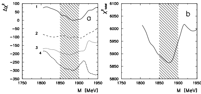
Fig. 16. The result of D_{13}(1870) mass scan. a) 1: d\sigma/d\Omega for \gamma p \rightarrow \pi^0 N (GRAAL); 2: the \Lambda K^+ recoil polarisation (CLAS); 3, 4: d\sigma/d\Omega for \gamma p \rightarrow \Sigma K reaction (SAPHIR, CLAS); b) the total \chi^2 for all \Lambda K^+ and \Sigma K reactions.
